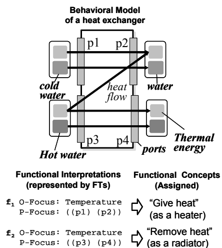
Figure 3. Functional interpretations of a heat exchanger
