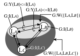
Fig. 2. Learning Goal Ontology
