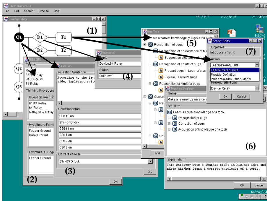
Figure1 Training Scenarios
