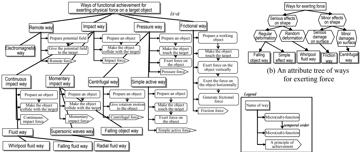
(a) An is-a hierarchy of ways for exerting force Figure 3. An is-a hierarchy and an attribute tree of ways of function achievement for “exerting physical force”
