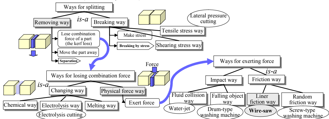
(c) A decomposed organization of the ways for cutting (portion) Figure 4. An example of organizing generic ways in is-a hierarchies.
