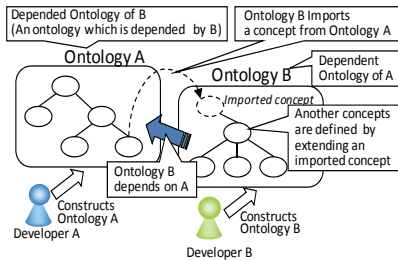
Fig. 1. Distributed Ontology Development.
