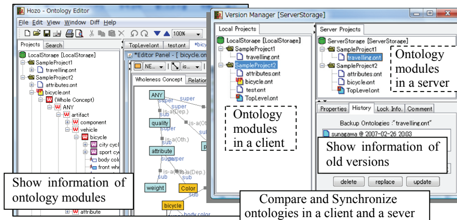
Fig.5. A snapshot of Ontology Manger.
