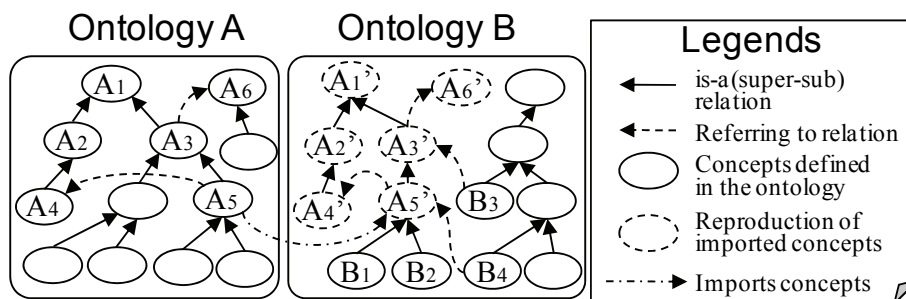
Fig.3. A framework for dependency management among ontologies.
