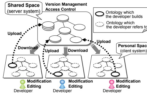
Fig. 2. A Conceptual Framework for Distributed Ontology Development.
