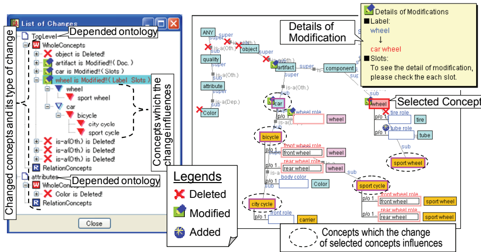
Fig. 6. Tracking Pane.
