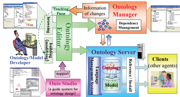
Fig.4. Architecture of Hozo
