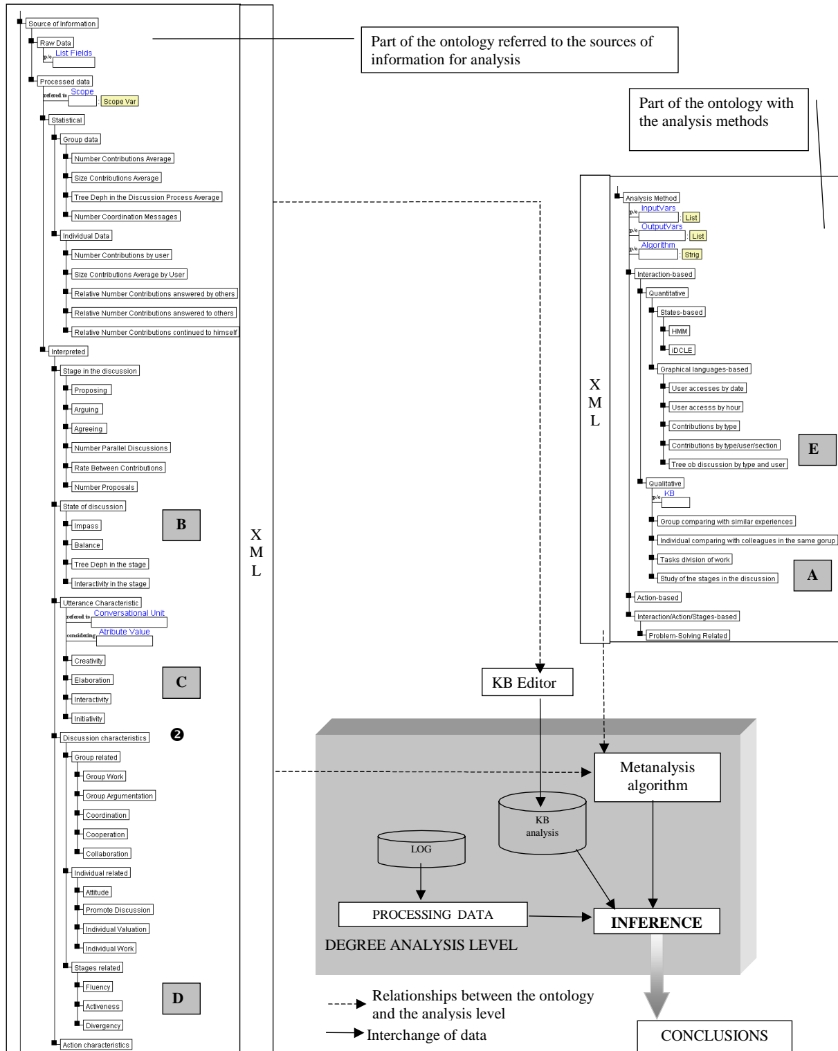
Figure 3. Relationship between the ontology contents and the analysis level in DEGREE system
