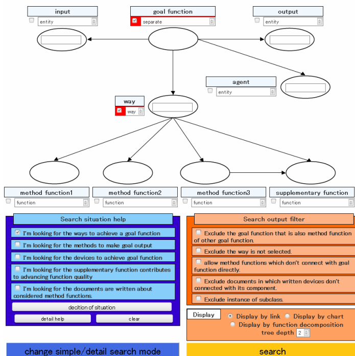
Figure 5: The interface of Funnotation search system.
