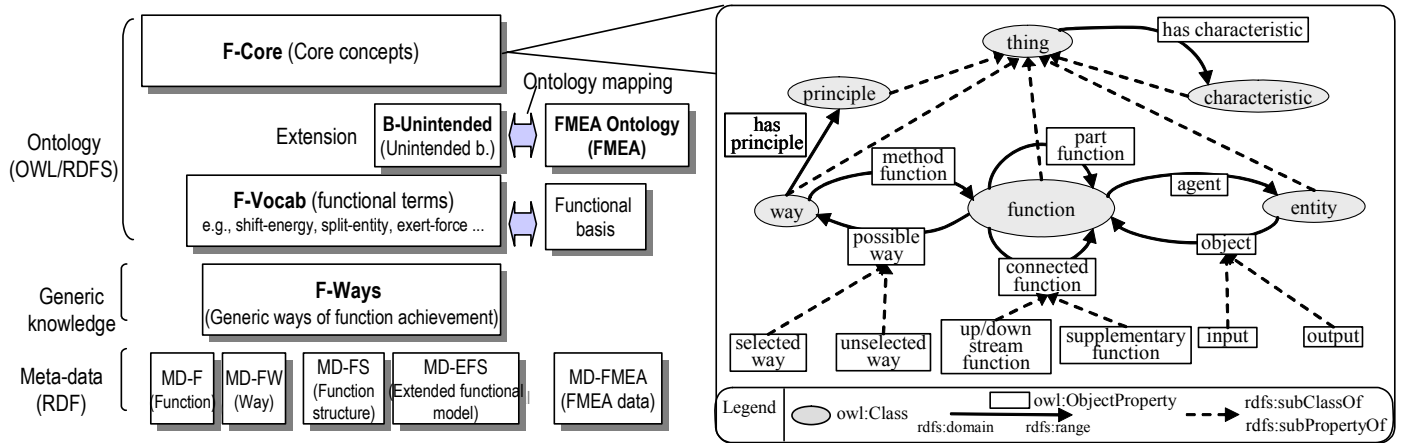
Figure 3: Layers of Funnotation Schema and the classes and the properties of F-Core (portion).
