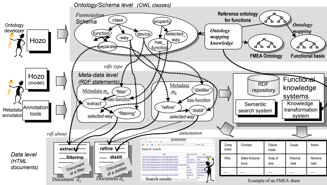
Figure 2: Overview of the Funnotation framework and systems.
