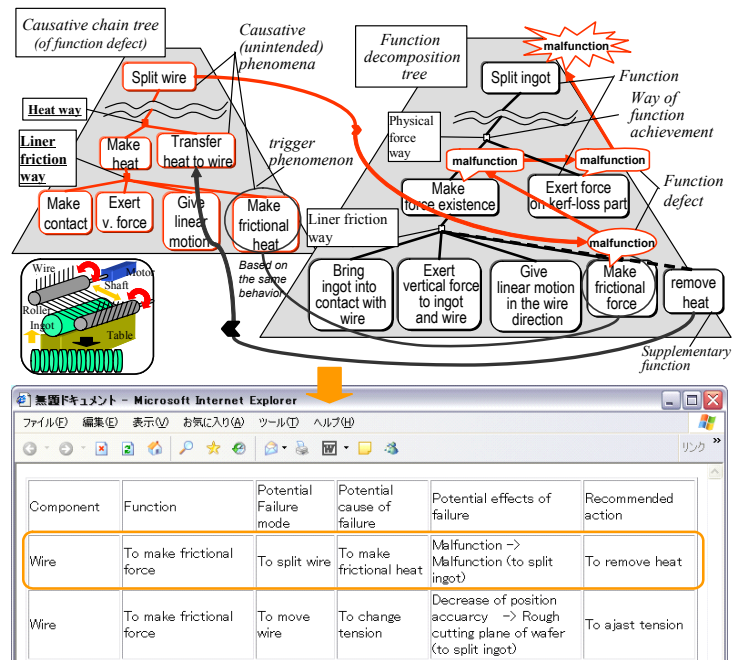
Figure 8: Example of knowledge transformation from an extended functional model to a FMEA document.
